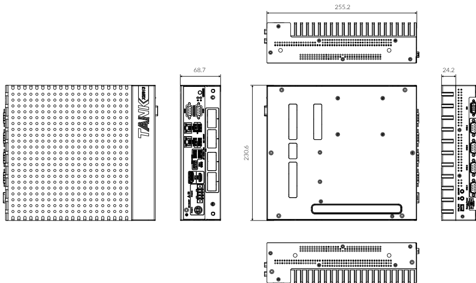
TANK-XM813
